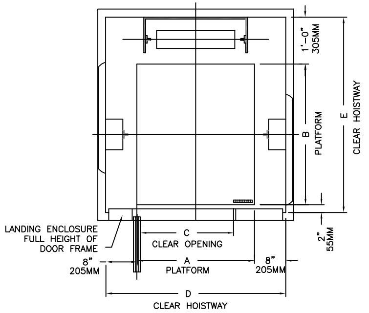
REAR COUNTERWEIGHT
