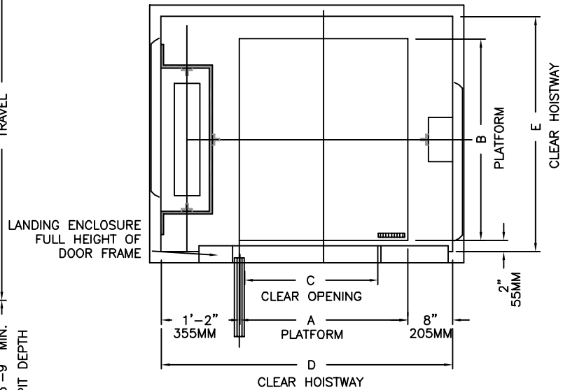
SIDE COUNTERWEIGHT MAY BE TO EITHER SIDE
